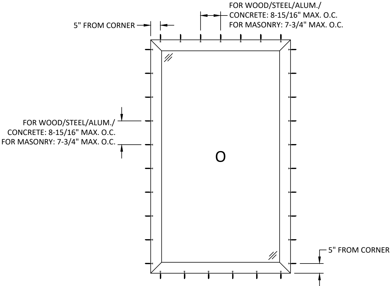
ANCHOR LAYOUT
