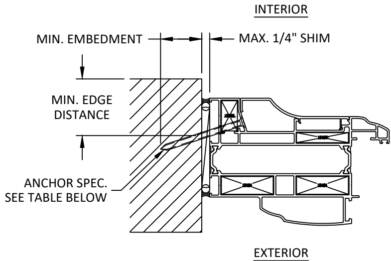
C 5 INSTALLATION DETAIL JAMB
