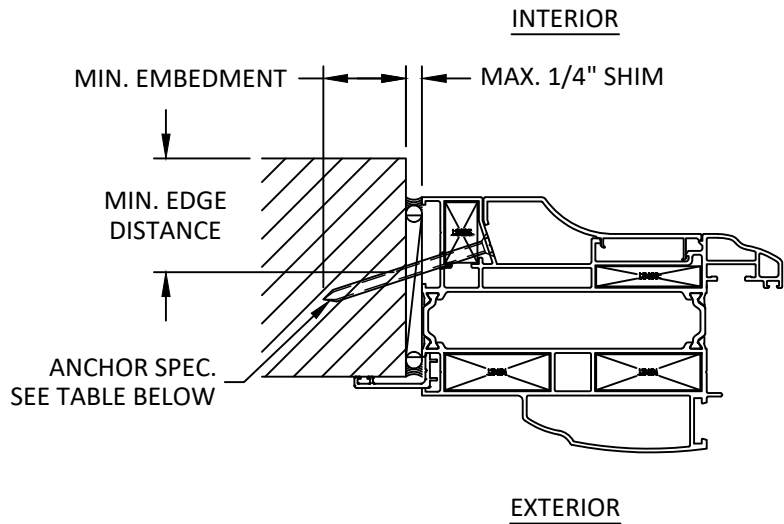
D 5 INSTALLATION DETAIL JAMB WITH FLANGE
